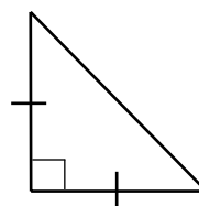
Right Triangle
